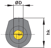
A...T Innere Kühlmittelzufuhr durch die Schneide Through coolant supply through the insert
